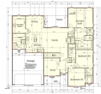
1 FIRST FLOOR PLAN
