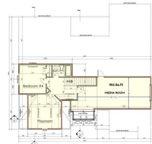
2 SECOND FLOOR PLAN
